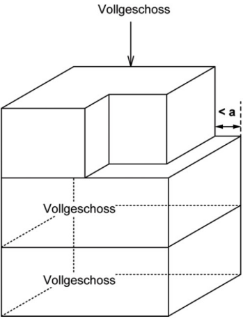
Figur 6.4 Attikageschosse
