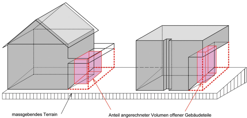
Figur 8.3 Baumassenziffer
